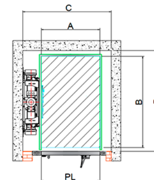
Entrada Unilateral
